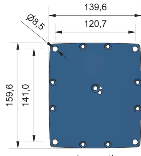
Outer profile bottom plate
