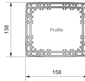
Inner profile top plate
